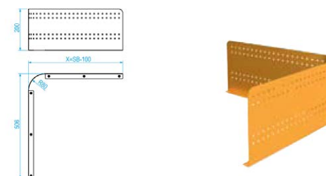
Tin shield h=200
