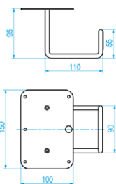
Hanger AK-AF0S
