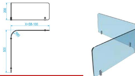
Plexiglass shield h=200
