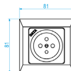
Socket ~ 230V DATA AK-P00000640
