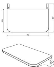
Rack 250x450 AK-PC0S
