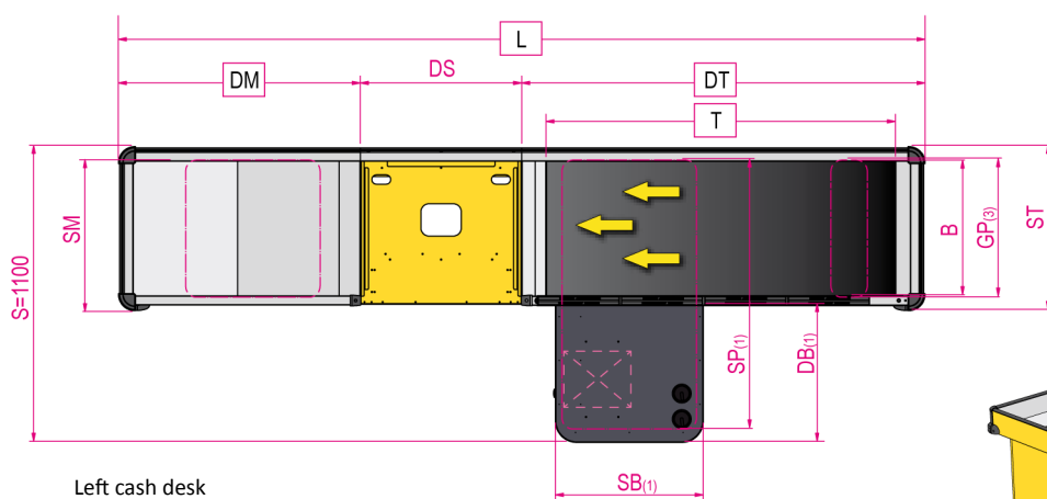
Left cash desk
