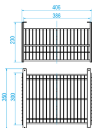
Basket H-230, G-300 AK-ABG0S
