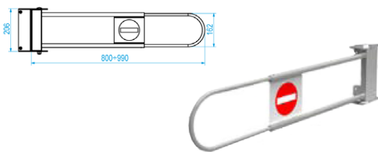
Gates AK-AG0S
