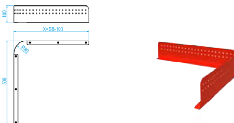
Tin shield h=100
