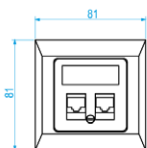
Network socket Ethernet AK-P00000645
