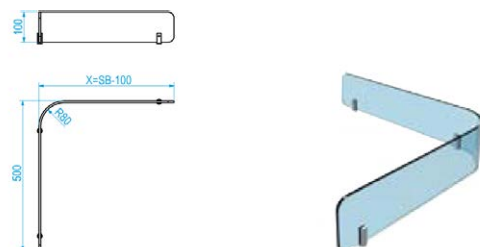
Plexiglass shield h=100
