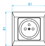
Socket ~ 230V AK-P00000500
